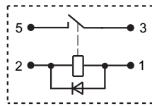
HFV6-G/12-H□□□-D1(XXX)
