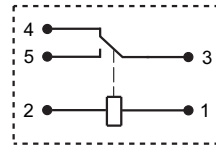
HFV6-G/12-Z□□□-R(XXX)
