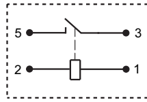
HFV6-G/12-H□□□-R(XXX)
