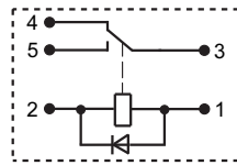
HFV6-G/12-Z□□□-D1(XXX)
